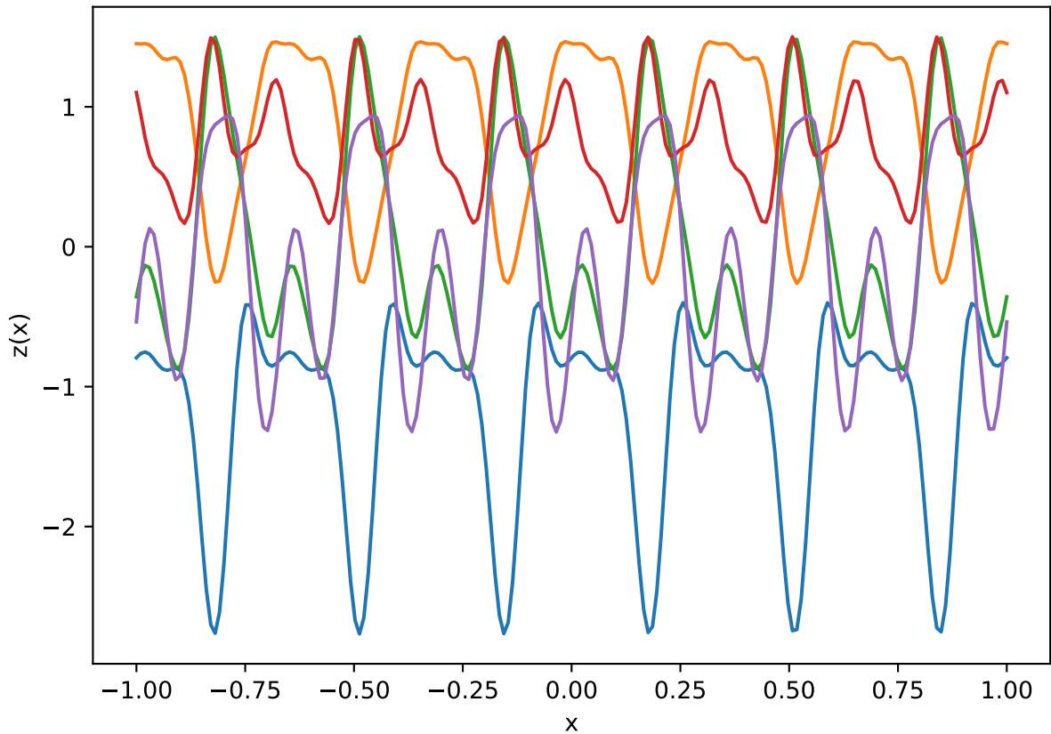
GP - Periodic kernel
